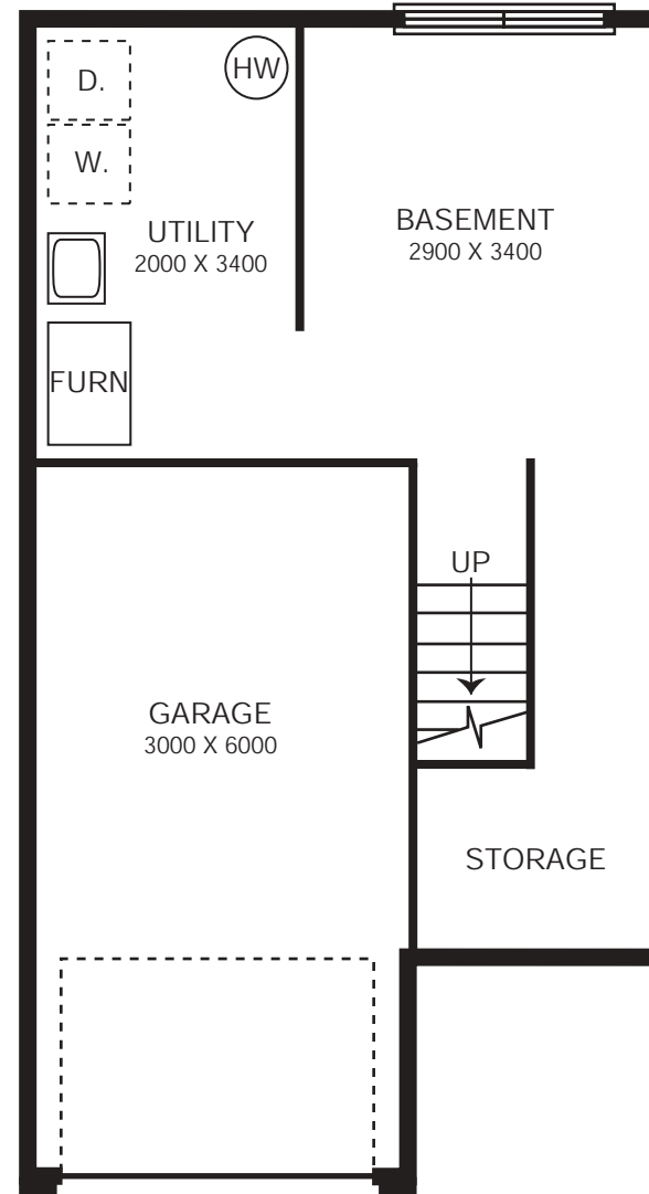
BASEMENT
