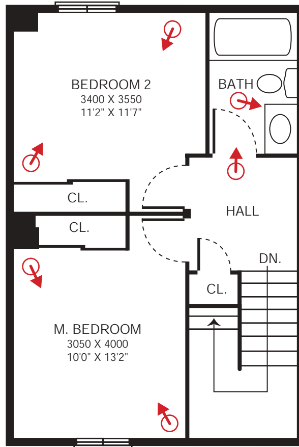
2ND FLOOR
