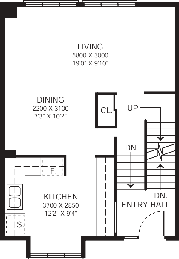
MAIN FLOOR
